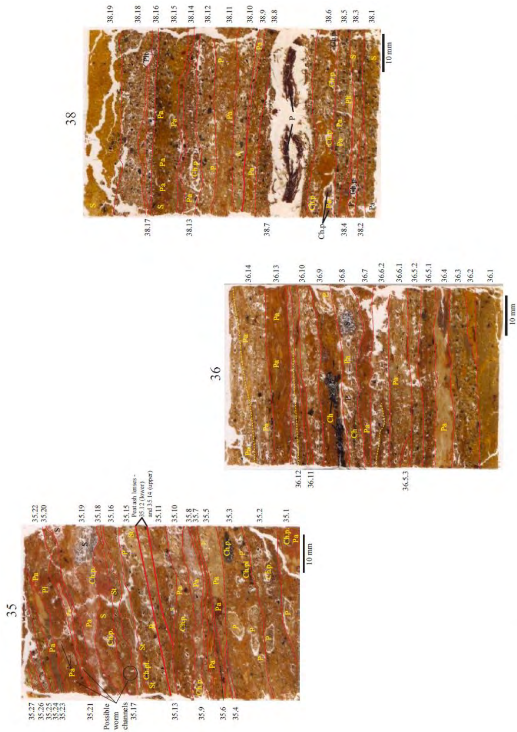
Figure 10 - Thin sections 06-35, 06-36 and 06-38 taken from occupation phase 1 in booth [2397] B=bone, Ch=charcoal, Ch.p=charred peat, S=fuel ash slag, P=peat, Pa=peat ash, Plt=Plant tissue, St=stone
