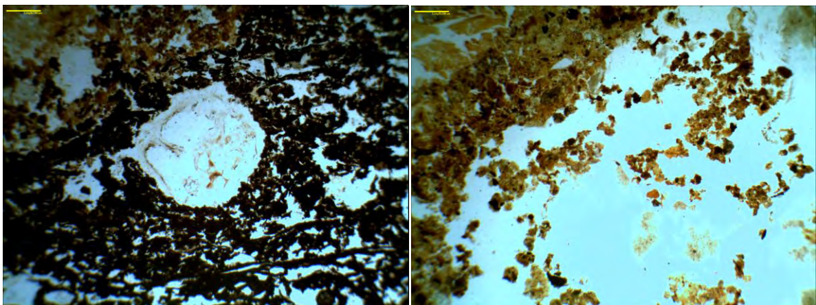
Figures 16 and 17 – Root nodule embedded in charred peat (left) from layer 40.5, excrement in a worm channel (right) from layer 8.14, scale bars about 200 \mu m.
