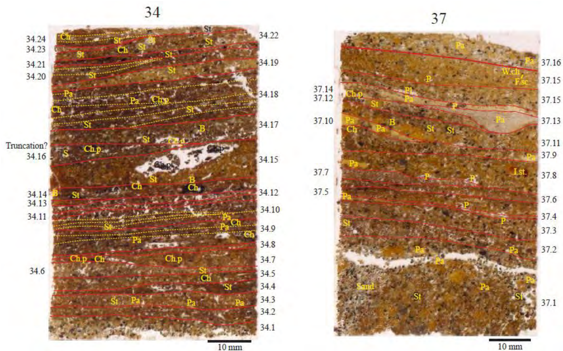
Figure 11 - Thin sections 06-34 and 06-37 taken from occupation phase 3 in booth [2397]
