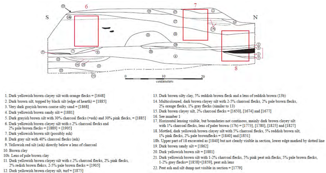
Figure 7 – Section drawing of sediment bulk in booth [1765] showing the positions of micromorphology samples 05-6 to 05-8
