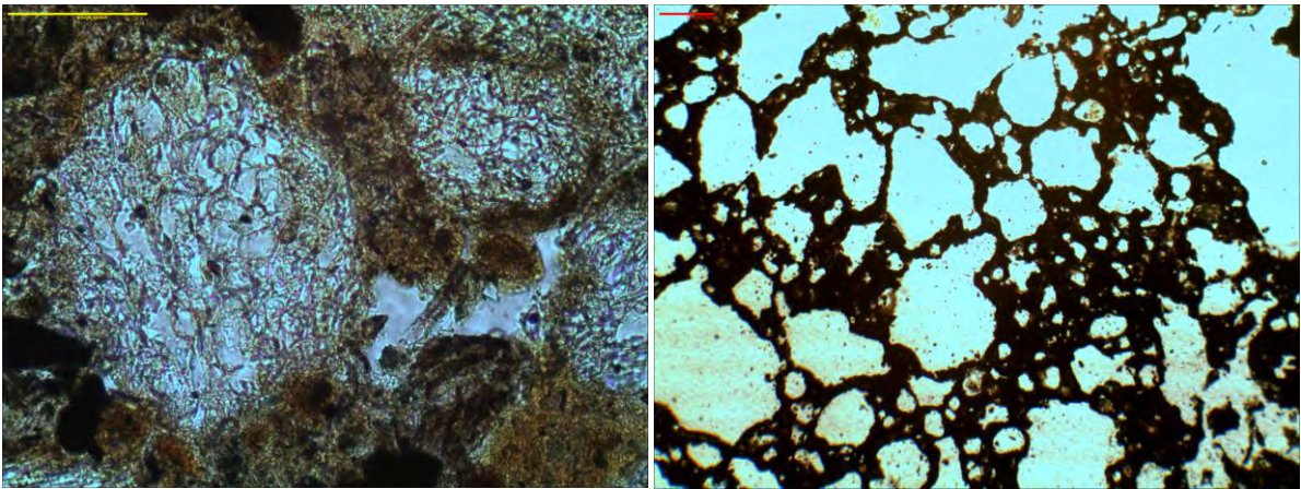
Figures 27 and 28 – Light fuel ash slag (left) from layer 39.13 and dark fuel ash slag (right) from layer 36.8, yellow scale bar about 100 \mu\text{m} , red scale bar about 200 \mu\text{m} .
