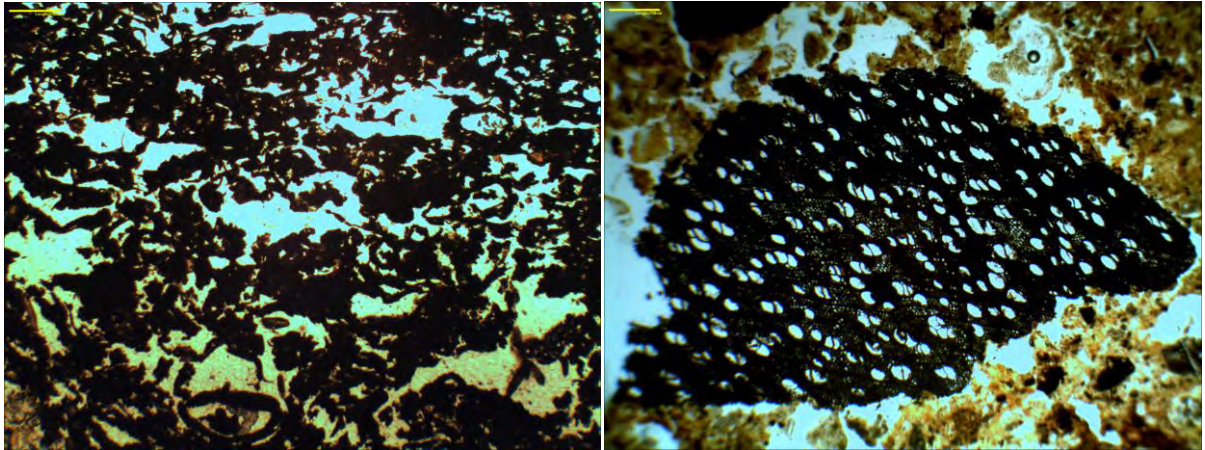
Figures 25 and 26 – Charred peat (left) from layer 40.5 and birch charcoal (right) from layer 8.14, scale bars about 200 \mu\text{m}
