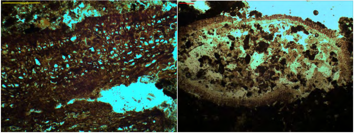
Figures 12 and 13 – Plant tissue (left) from layer 39.14, bark (right) from layer 39.7, scale bars about 200 \mu m
