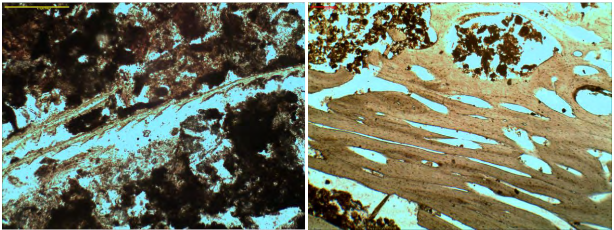
Figures 14 and 15 – Fish bone (left) from layer 39.15, calcined bone (right) from layer 40.5, scale bars about 200 \mu m.
