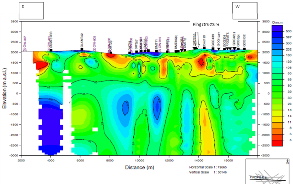
FIGURE 7: East West Cross section along Profile 5 in Olkaria Geothermal Field cutting across the ring structure
