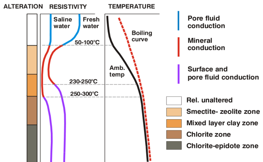
FIGURE 5: General resistivity structure of a high-temperature geothermal system showing resistivity variation with alteration and temperature (modified from Árnason et al., 2000)
