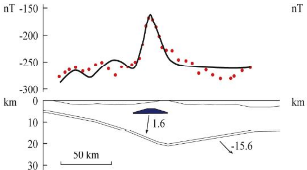
FIGURE 3: A cross section showing a 2D body modelled to fit the observed magnetic field anomaly. The red dots show observed field while the black line show the calculated field
