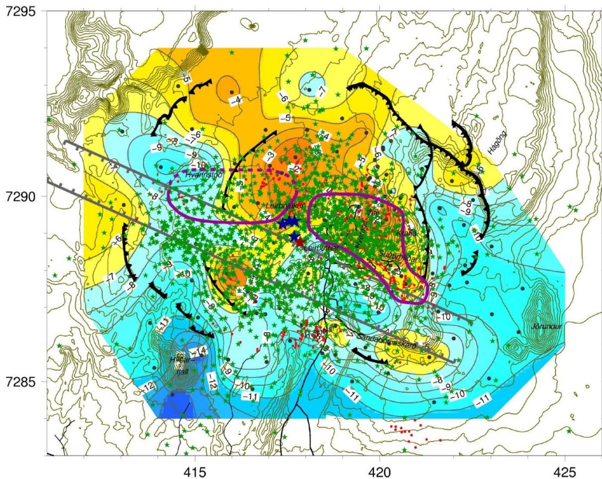
FIGURE 10: Elevation (km above sea level) of the top of conductors within the crust of Krafla, geological features inferred from gravity data (the inner caldera, black hatched lines and the oblique rift graben, gray fault lines), epicentres of earthquakes (green stars), boundaries of S-wave shadows (purple lines), centres of crustal deformation in 1984 (blue stars) and centre of subsidence from 1992 to 1995 (red star).
