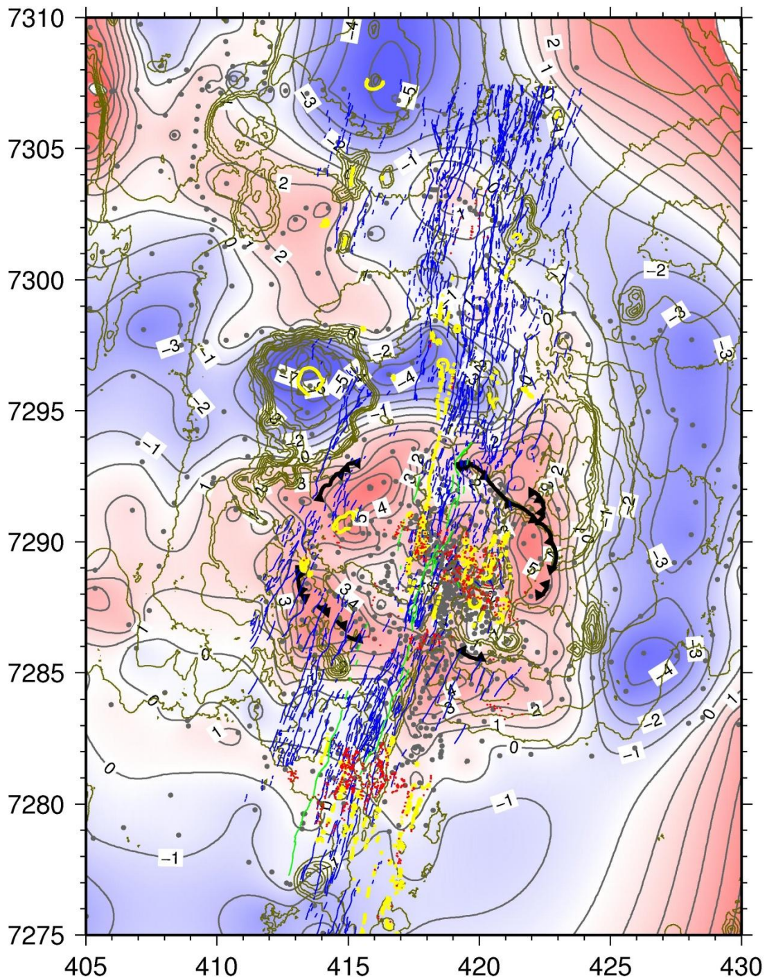
FIGURE 1: De-trended Bouguer gravity map (mgals) of Krafla and surrounding areas. Faults and fissure (blue), the caldera (hedge black lines) eruptive fissure and craters (yellow) and geothermal surface manifestations (alteration, hot springs and fumaroles, red). Boundaries of the part of the fissure swarm that was active in Krafla fires are shown as green lines. The topography (elevation contours) is shown with brown lines.
