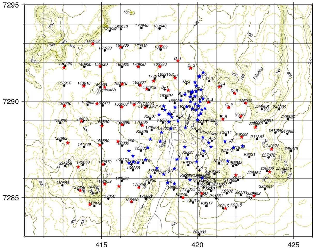
FIGURE 6: Location of interpreted MT soundings. Blue stars are soundings made in 2004 and 2005. Red stars are soundings made in 2006. TEM soundings are shown as black dots.
