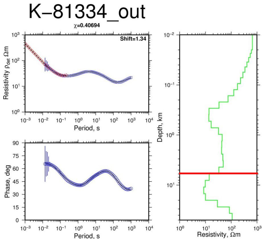
FIGURE 5: A typical result of a joint inversion of TEM and MT soundings. Red circles are the measured TEM apparent resistivity values and the blue circles are the apparent resistivity and phase values derived from the determinant of the impedance tensor. Black solid thin lines are calculated responses of the model to the right. In order to make the MT apparent resistivity tie in with that of the TEM, the MT apparent resistivity values have to be divided by a shift parameter of 1.34 (top right corner of the apparent resistivity panel).
