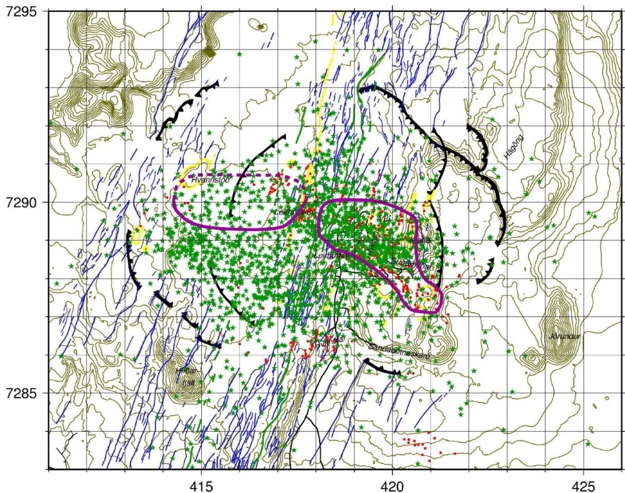
FIGURE 4: Earthquake epicentres (green stars) and boundaries of S-wave shadows (purple lines) observed during the Krafla fires (reproduced from Einarsson, 1991). Other geological features are the same as on previous maps.
