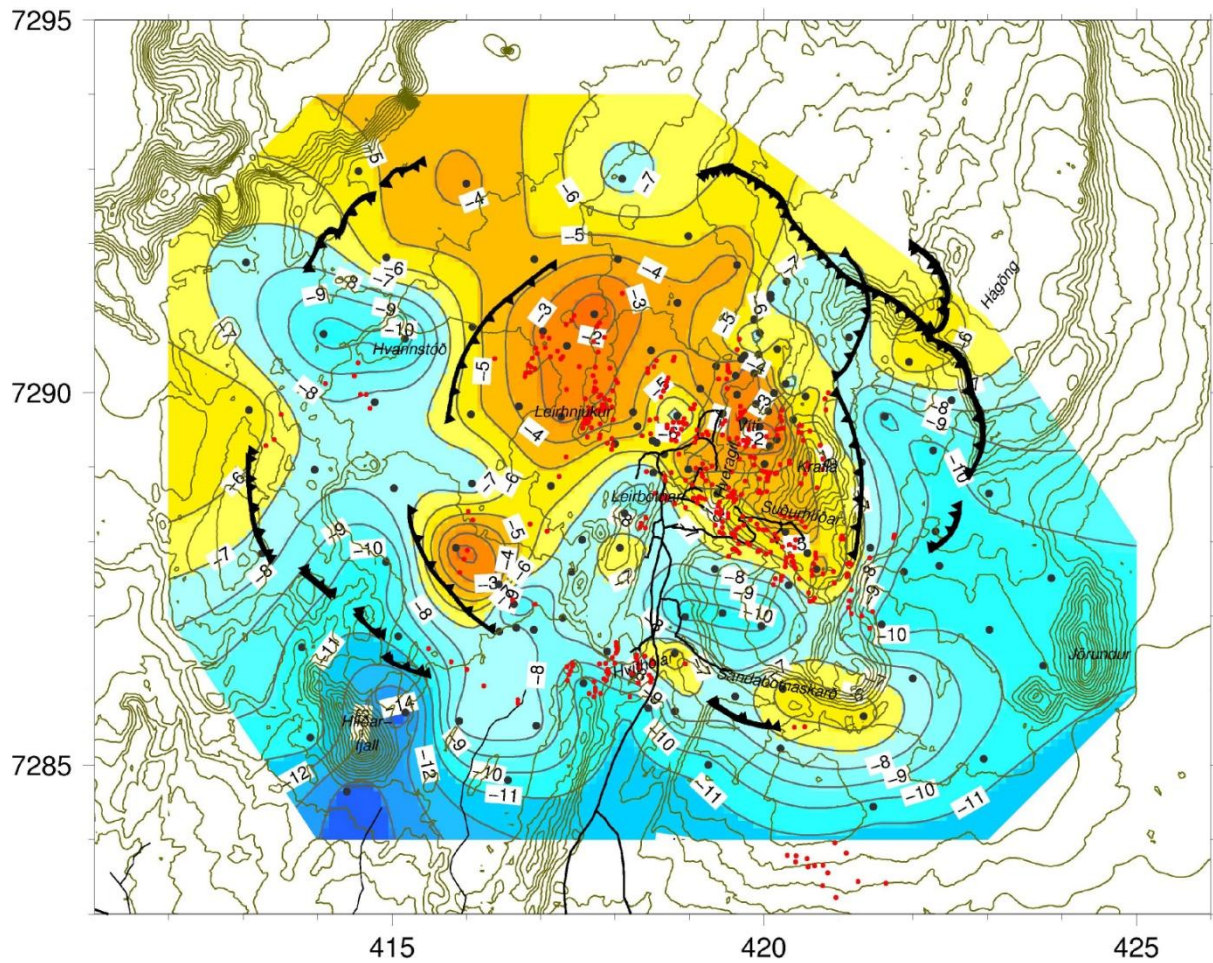
FIGURE 8: Elevation (km above sea level) of the upper boundary of deep conductors in the Krafla volcanic complex. Caldera rims are shown by black hatched lines and geothermal surface manifestation by red dots.
