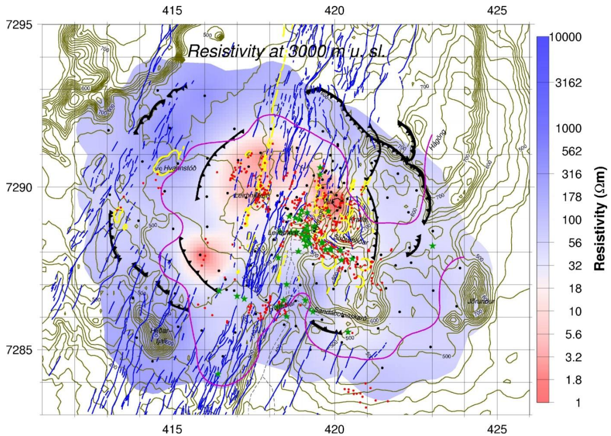
FIGURE 7: Resistivity at 3 km below sea level. The boundaries of the resistive core at 600 m b.s.l. are shown by a purple line.
