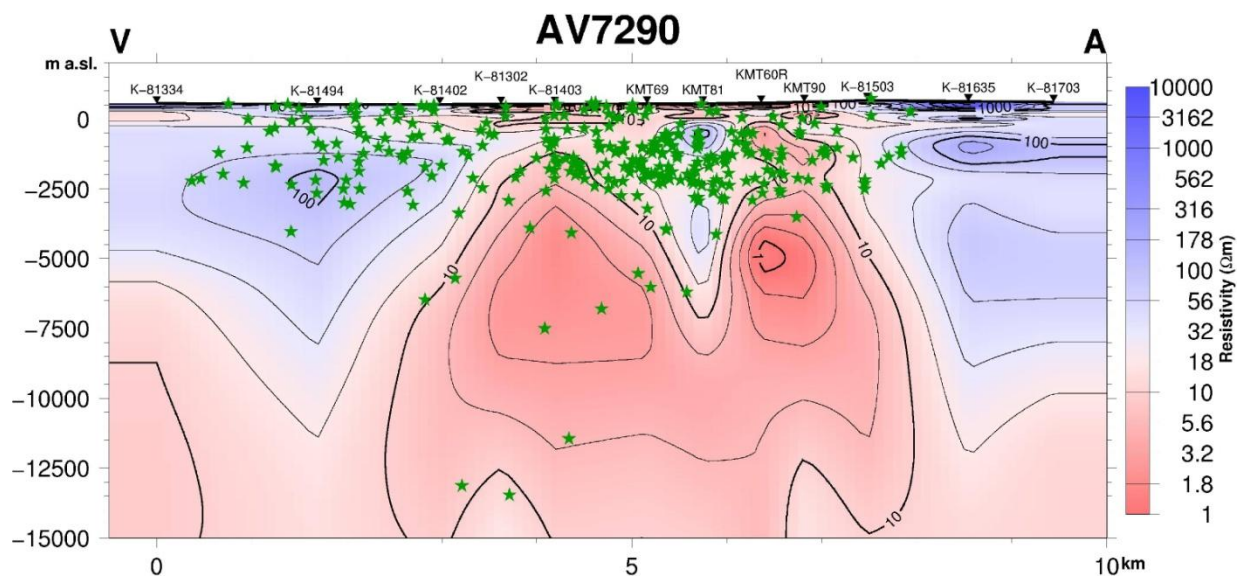
FIGURE 9: E-W cross-section AV7290. Located immediately south of line 7290 (see Figure 7). Earthquakes at distances less than 500 m are projected on the section (green stars).
