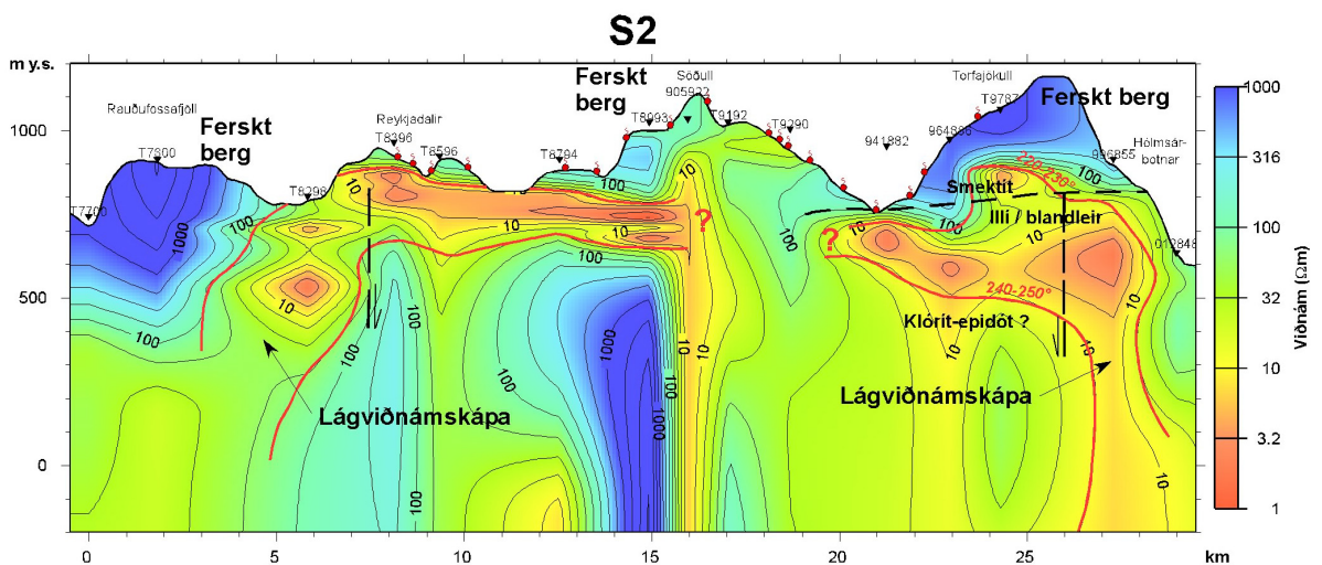
FIGURE 7. East-west section showing resistivity and its inferred correlation with alteration zoning. The alteration of the accessible uppermost few hundred metres gives a tie to conclude about the kind of alteration which causes the resistivity below.
