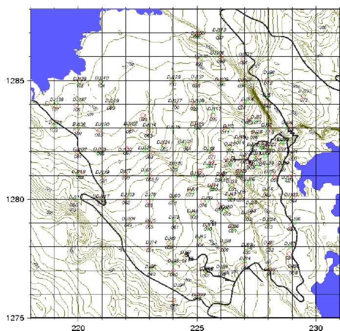
FIGURE 5: TEM and MT surveys of Asal rift (REI-ISOR 2008)
