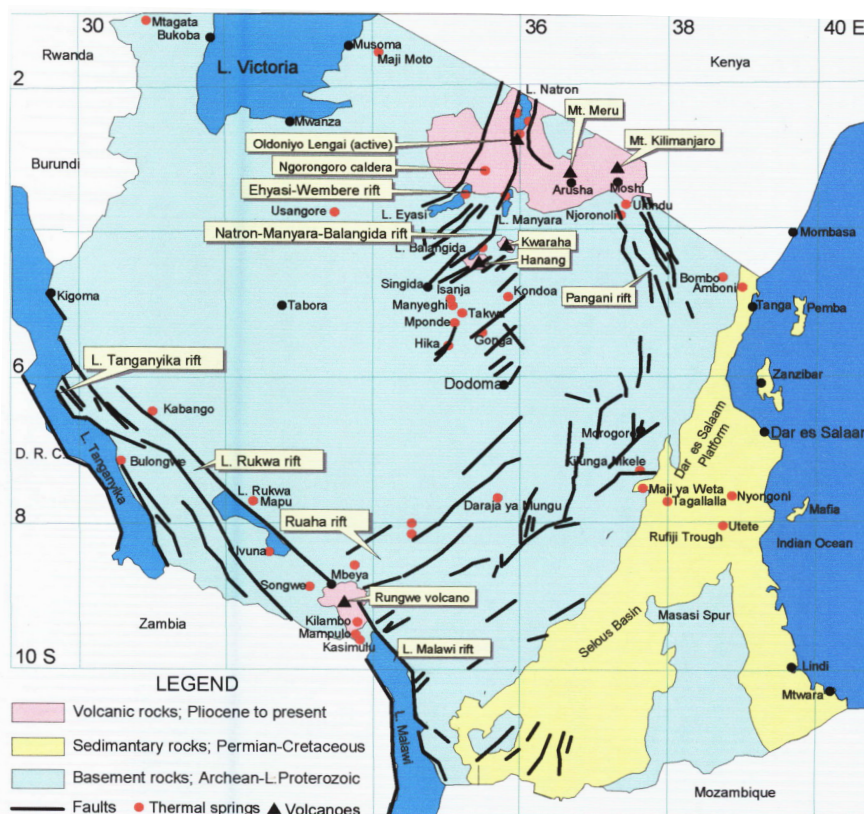
FIGURE 2: Geothermal sites in Tanzania
