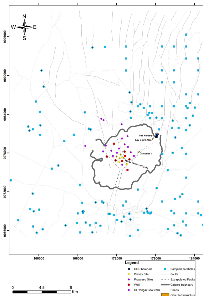
FIGURE 4: Location of boreholes considered for the geohazard monitoring study in the Menengai geothermal field
