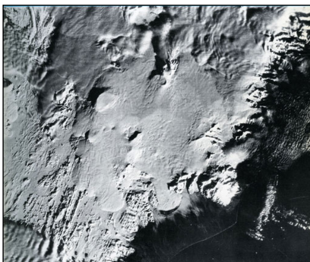
FIGURE 3: Vatnajökull glacier (9500 km 2 ) is located in the smooth field in central part of the figure. Two central volcanoes with calderas were first recognized in its NW and SE part from this image. A third caldera to the north of these was also recognized here for the first time.
