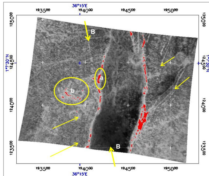
FIGURE 9: Thermal ortho-image of Area B
