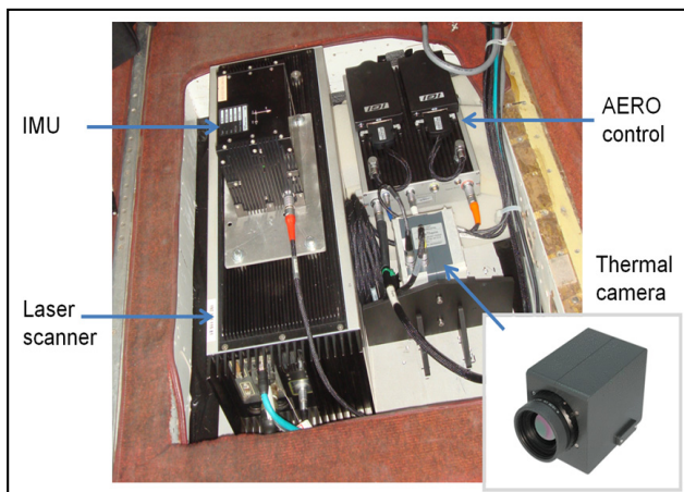
FIGURE 2: Thermal system equipment layout in the aeroplane
