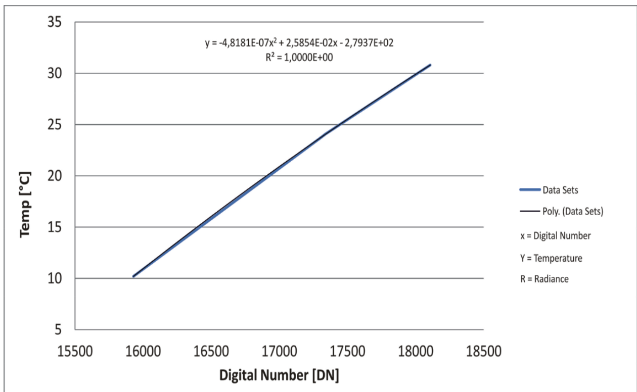
FIGURE 5: Temperature range function developed to convert 16 bit digital number values of pixels of single thermal images and of thermal mosaic to temperature values
