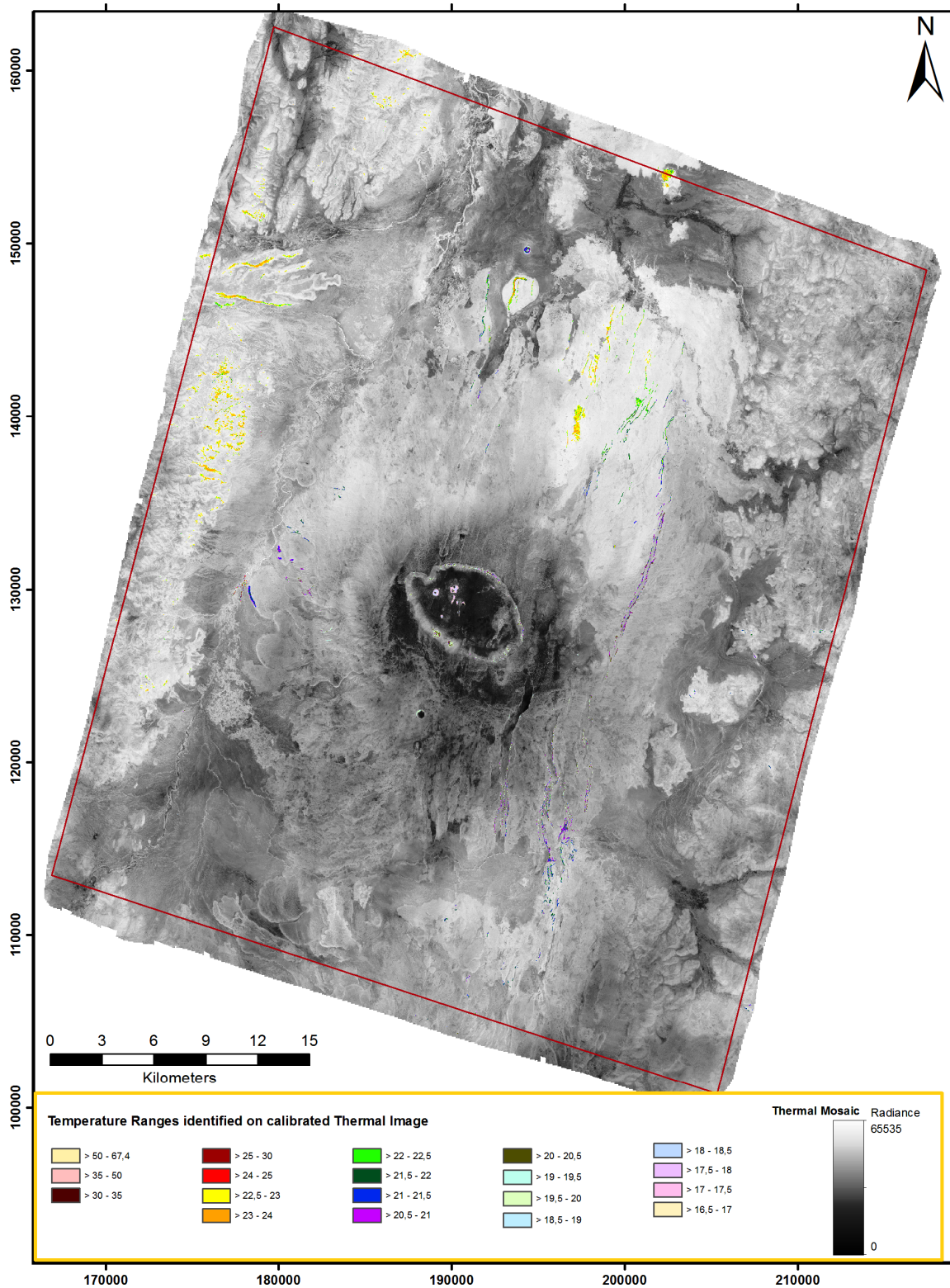
FIGURE 6: Thermal anomalies from the mosaicked image
