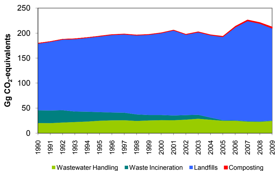
Figure 2.22: Emissions of greenhouse gases in the Waste sector 1990-2009 in Gg CO 2 -equivalents.
