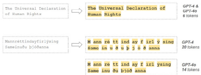
Tokenization efficiency for Icelandic has improved significantly in newer GPT models but still lags behind English.
