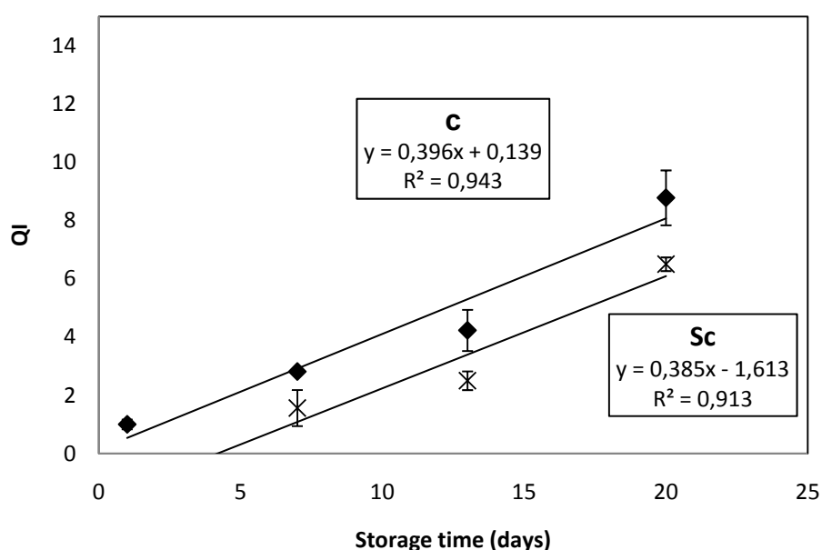
Figure 6: Quality index of de-skinned tilapia fillets using original scheme. Averages ( \pm SD) over each day analysed (N=3 per group) during storage. \blacktriangle = chilled at 1^{\circ}\text{C} (C); \times = superchilled at -1^{\circ}\text{C} (Sc)
