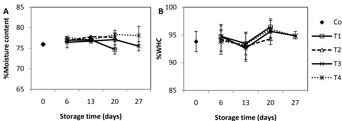
Figure 28: Changes in moisture content (A) and water holding capacity (WHC) (B) in packaged tilapia fillets during storage. Co= control; T1= 100% air, stored at 1°C; T2= 100% air at -1°C; T3= MA at 1°C; T4= MA at -1°C. Values (percentage of sample weight) are given as mean (N = 2).
