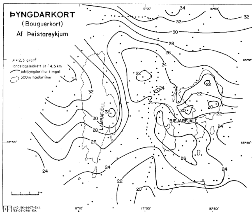
FIGURE 5: Bouguer map of Theistareykir. Values for iso-gravity lines are given as mgal. From Gíslason et al. (1984)
