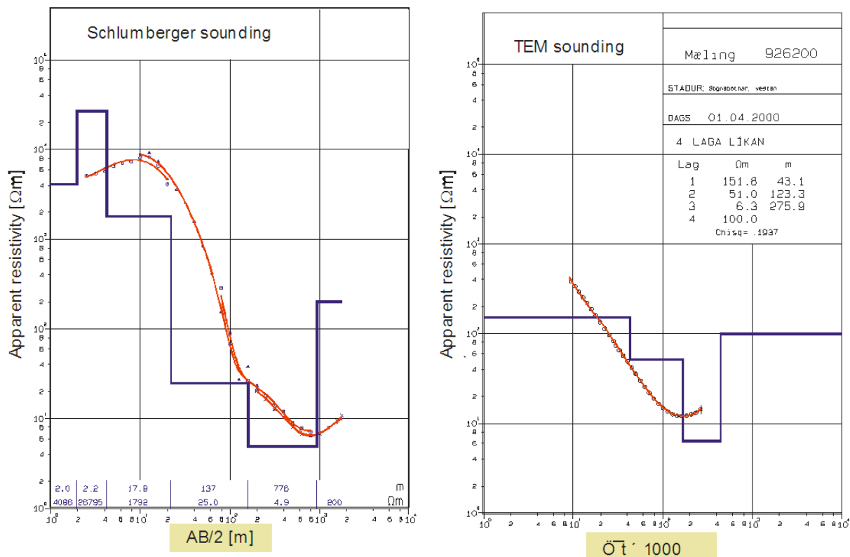
FIGURE 3: Curves showing a typical Schlumberger sounding (left) and a TEM sounding (right) and 1D models for their interpretation
