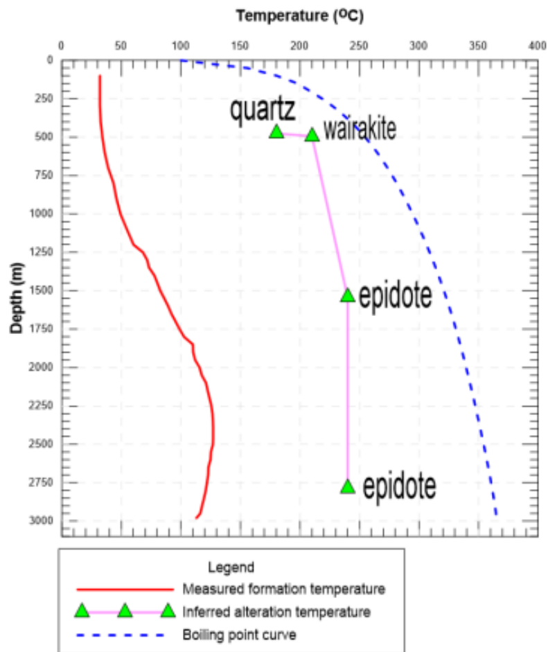
FIGURE 7: Comparison between formation, alteration minerals and boiling point temperature of well OW-922 (Otieno, 2016)
