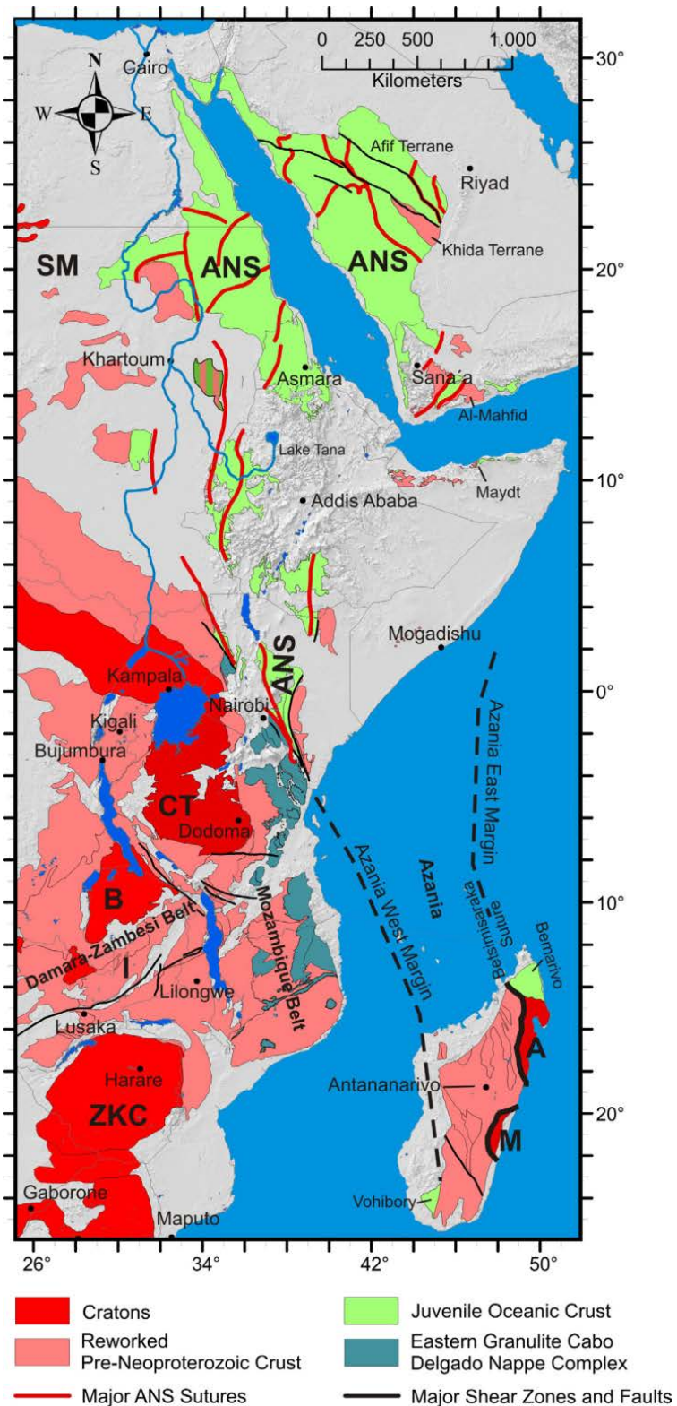
FIGURE 10: Distribution of crustal domains in the East African Orogen. SM, Sahara Metacraton; CTB, Congo–Tanzania–Bangweulu Cratons; ZKC, Zimbabwe–Kalahari Cratons; I, Irumide Belt; A, Antogil Craton; M, Masora Craton; ANS, Arabian Nubian Shield.
