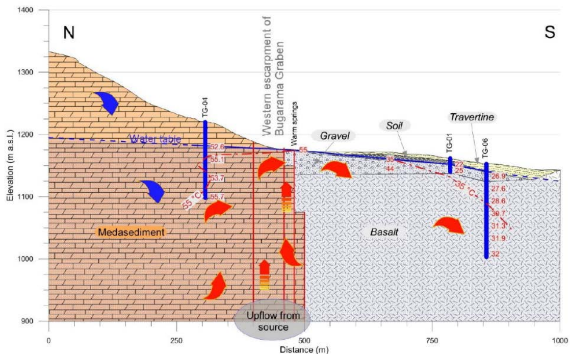
FIGURE 7: Conceptual model of the Bugarama geothermal area (Gíslason, 2016)
