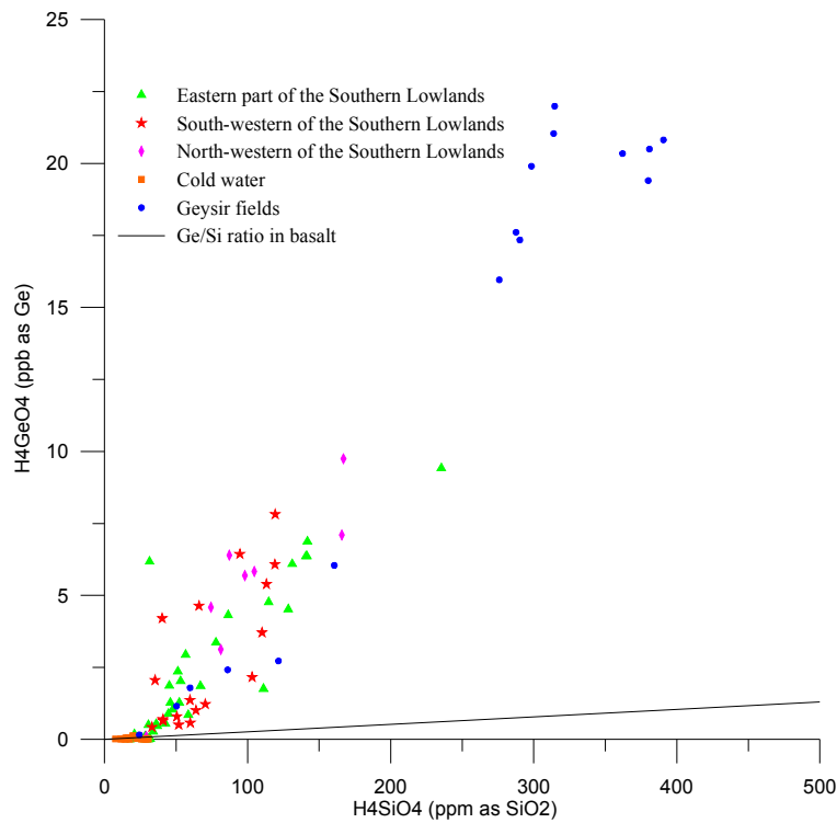
FIGURE 7: The relationship between Ge and Si in geothermal waters in the low-temperature field of the Southern Lowlands of Iceland and the Geysir field; the near-horizontal black line represents the Ge/Si ratio in basalts
