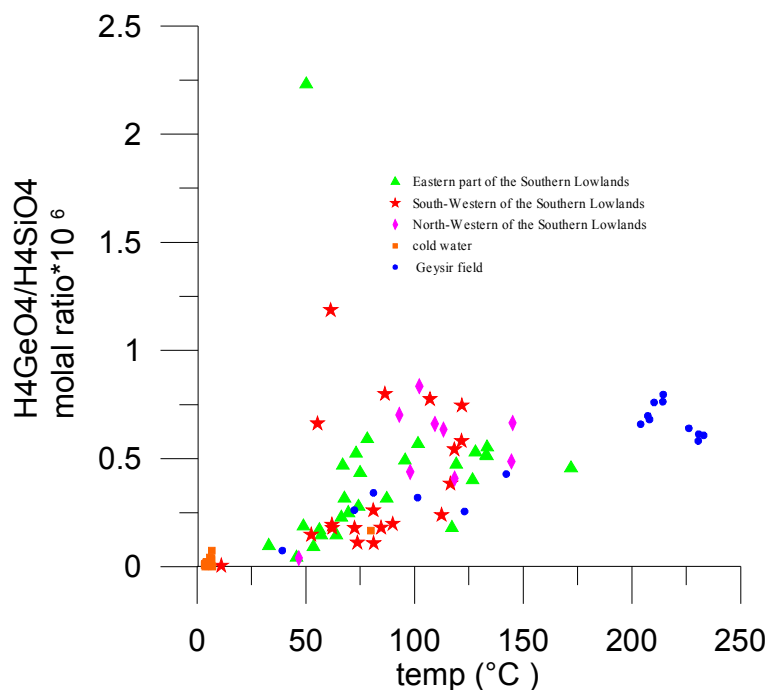
FIGURE 5: H_4GeO_4/H_4SiO_4 species ratios versus aquifer temperature in ground water and geothermal waters in the Southern Lowlands and the Geysir field; for selection of aquifer temperature see Figure 3
