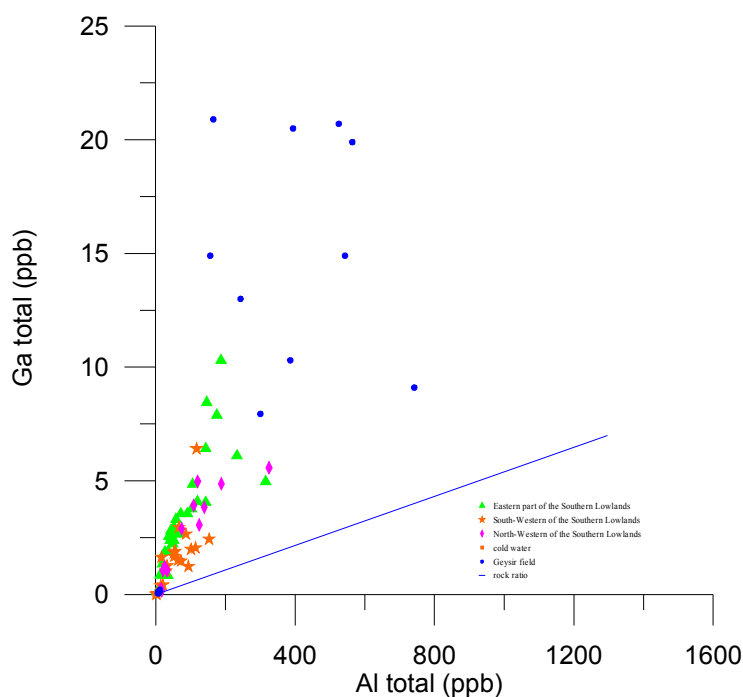
FIGURE 9: The relationship between Ga and Al in geothermal waters in the Southern Lowlands and the Geysir field; the gray (blue) line represents the average Ga/Al ratio in basalt
