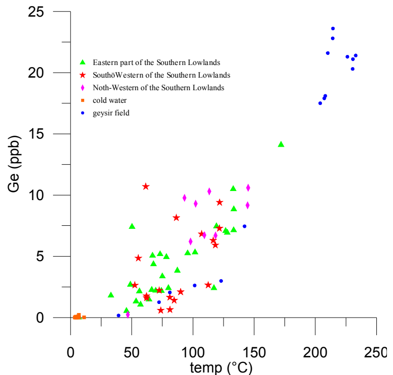
FIGURE 3: Germanium concentrations in geothermal waters as a function of aquifer temperature. For the high-temperature waters of the Geysir field, this temperature was taken to be represented by the quartz geothermometer but for the mixed waters in this field as well as in the low-temperature systems by the chalcedony geothermometer. For non-thermal groundwaters the measured temperature was used for reference
