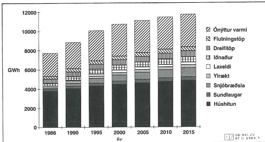
Possibilities for co-utilization of hydro and geothermal energy in Iceland.
