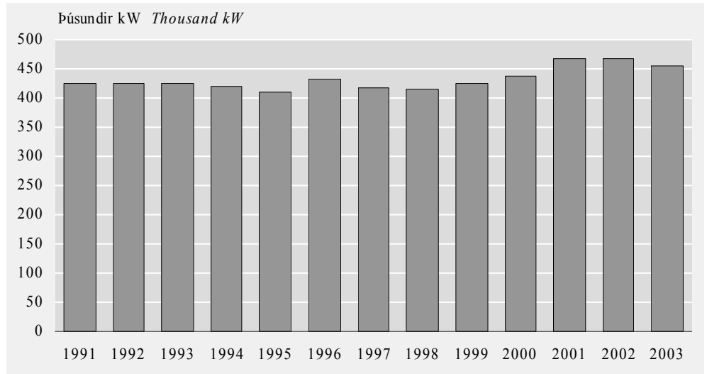
Figure 4. Decked vessels and trawlers 1991–2003. Power of main engine
