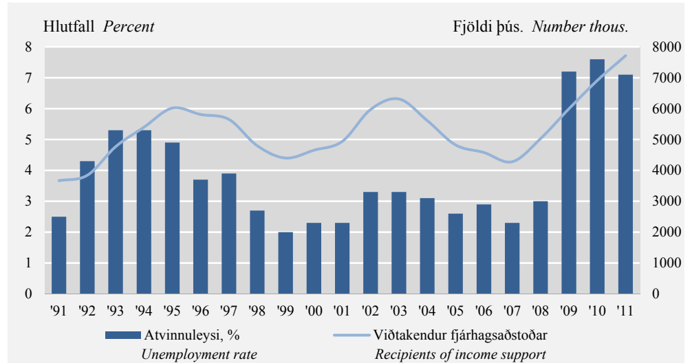
Figure 1. Unemployment rates and number of recipients of income support 2001–2011
