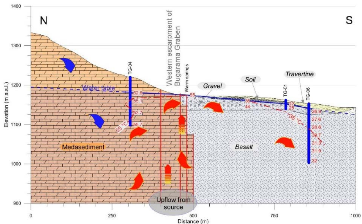
FIGURE 1: Conceptual model of the Bugarama geothermal area (Reykjavik Geothermal, 2016)
