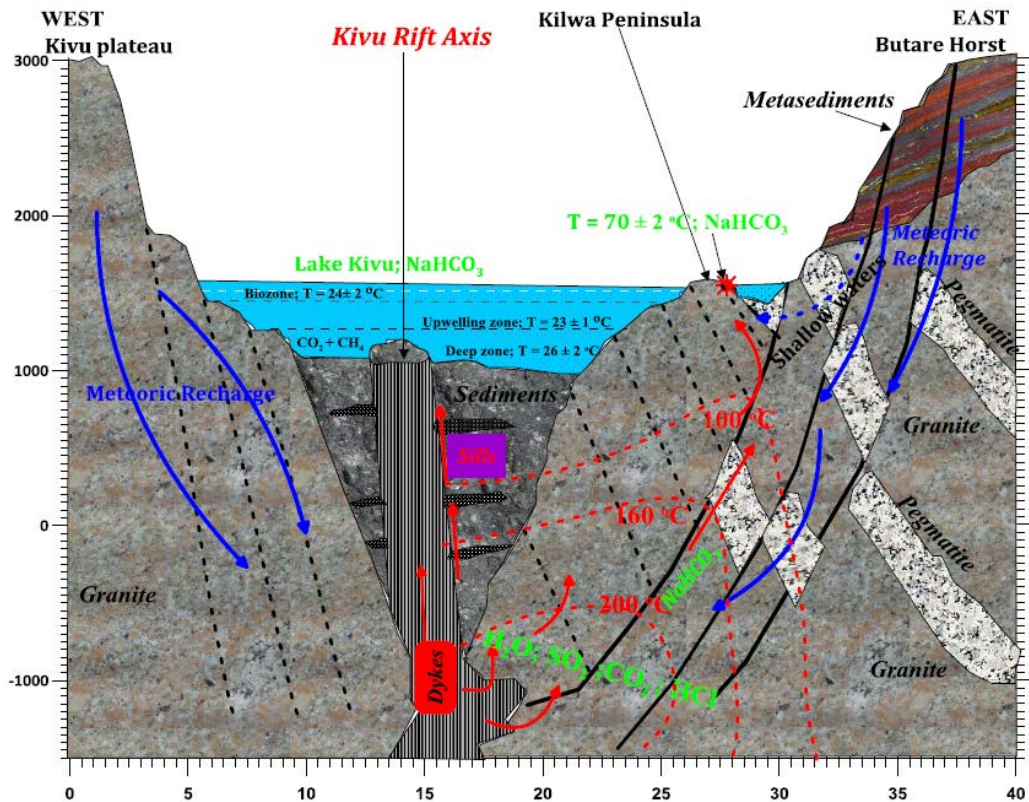
FIGURE 6: Conceptual geothermal model for Kilwa area (GDC and SARL Géo2D, 2017)
