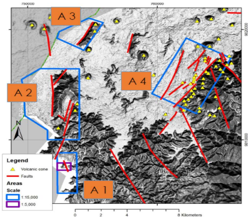
FIGURE 5: Geothermal target areas in Gisenyi prospect (GDC and SARL Géo2D, 2016)
