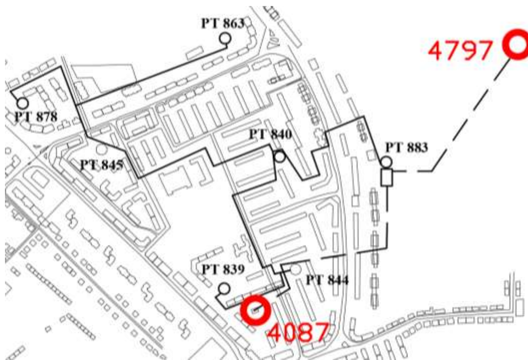
Figure 11: Layout of the existing system in Nufarul
