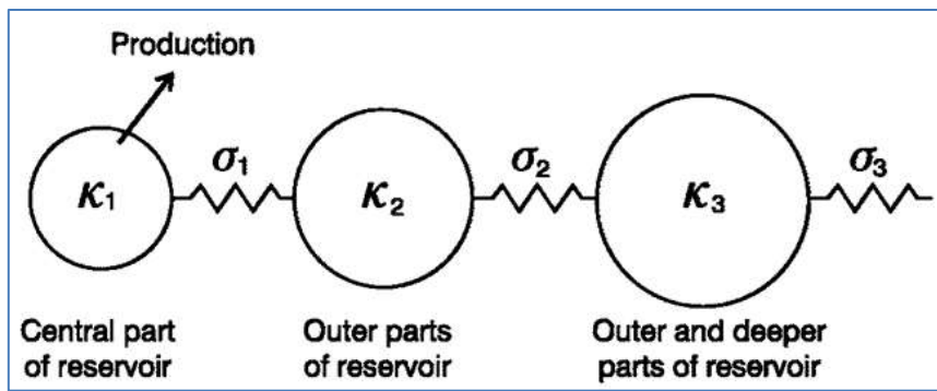
Figure 3: A 3-tank lumped ladder model commonly used to simulate geothermal systems (Axelsson et al., 2005)
