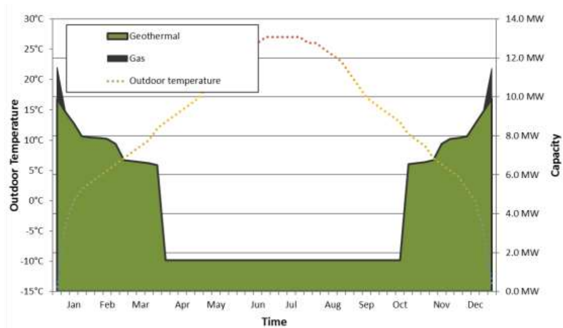
Figure 19: Heat demand and heat supply in Scenario 3
