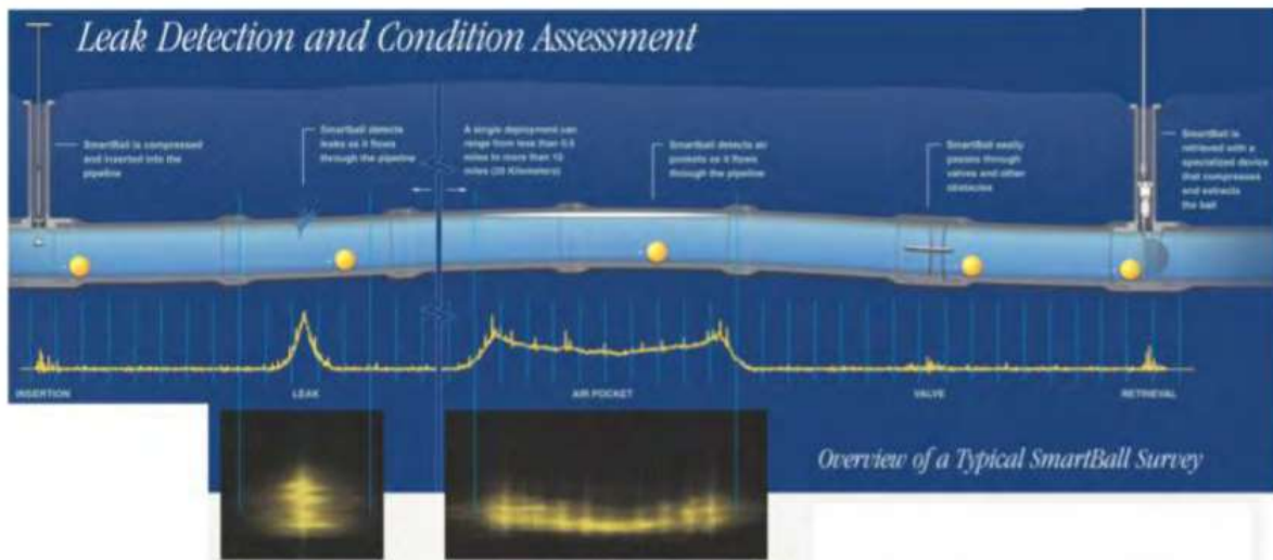
Figure 23: Overview of a typical SmartBall survey
