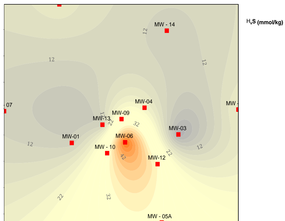
FIGURE 23: H 2 S distribution in Menengai wells
