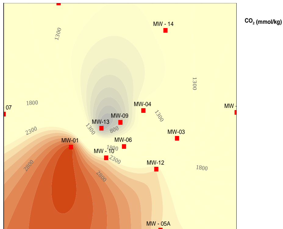
FIGURE 22: CO 2 distribution in Menengai wells
