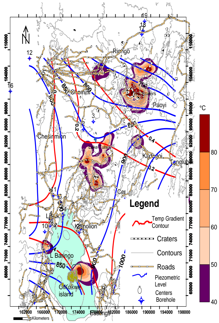
FIGURE 9: Temperature gradient and piezometric levels
