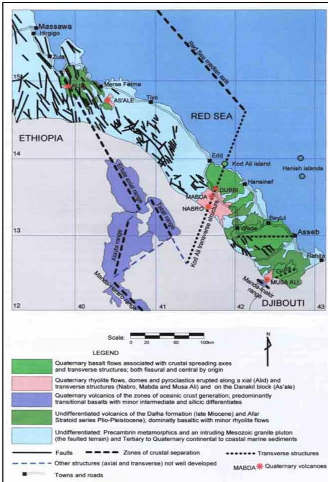
FIGURE 2: Regional geologic setting of the area
