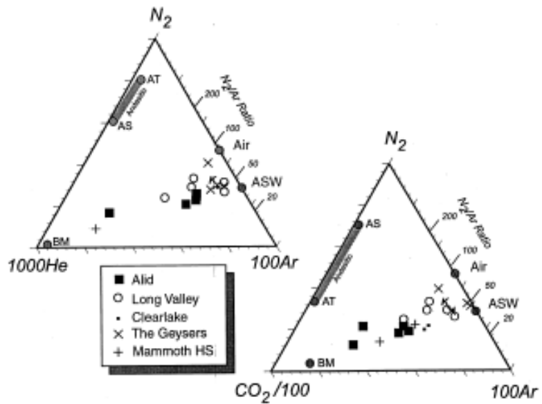
FIGURE 12: Triangular diagrams of N 2 vs 1000He vs 100Ar and N 2 vs CO 2 /100 vs 100Ar for fumarolic samples of Alid volcanic center. Fumaroles from non arc hosted geothermal systems are plotted for comparison (Lomenstern, 1999). The samples trend from an end-member of air saturated groundwater (ASW) contaminated with air towards a mantle end-member composition. BM, AS, AT and k, denote end member basaltic mantle, andesitic subducted, andesitic thermogenic and Olkaria sample, respectively. Samples are from Giggenbach, (1992).
