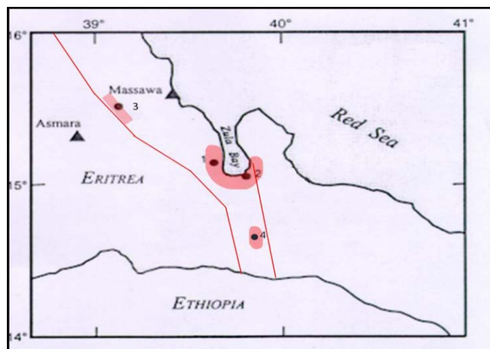
FIGURE 8: Location map of low temperature geothermal areas; symbols 1 and 2 are arou Gulf of Zula, 3 on the Asmara-Massawa road and 4 on Danakil Depression
