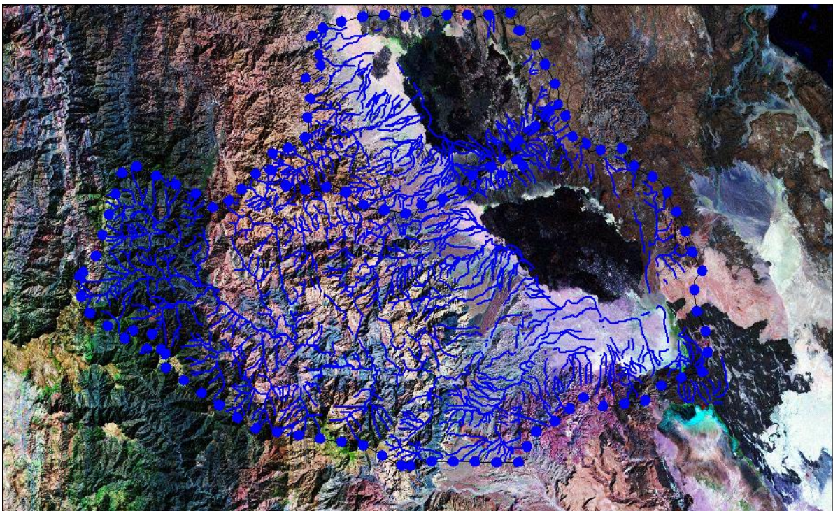
FIGURE 10: Catchments flowing to Alid: a) Wengebo (northern part); b) Alid (the Alid dome); and c) Samoti (southern catchment)
