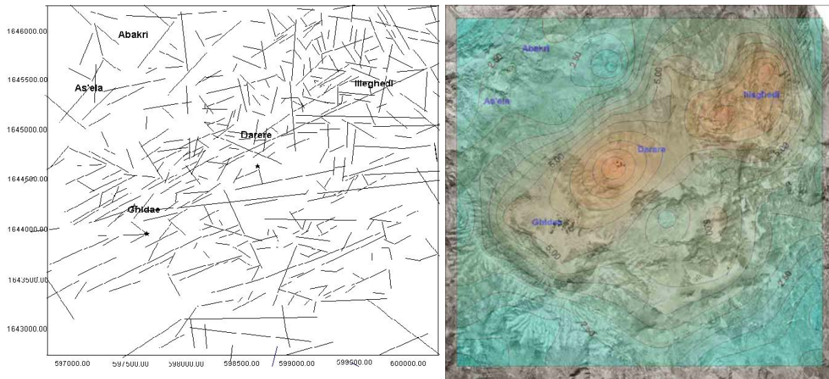
FIGURE 11: a) Lineaments interpreted mainly from aerial-photo and digital images of Alid; and b) Contour plot using FFD analysis
