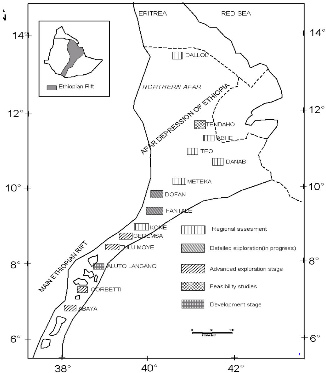
FIGURE 2: Location of geothermal prospects in Ethiopia
