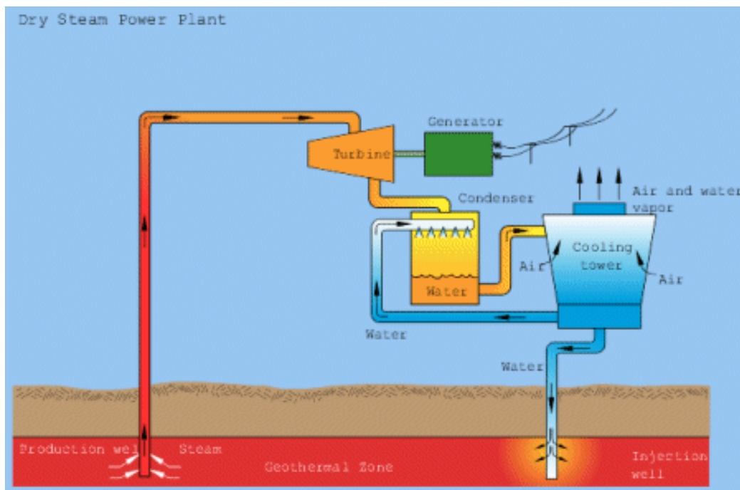
FIGURE 2: Schematic of a dry steam power plant
